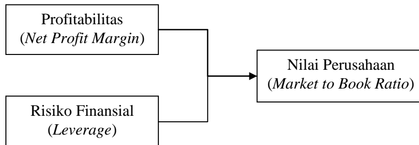
Gambar 1. Model Penelitian
