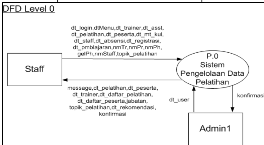
Gambar 6. DFD level 0
