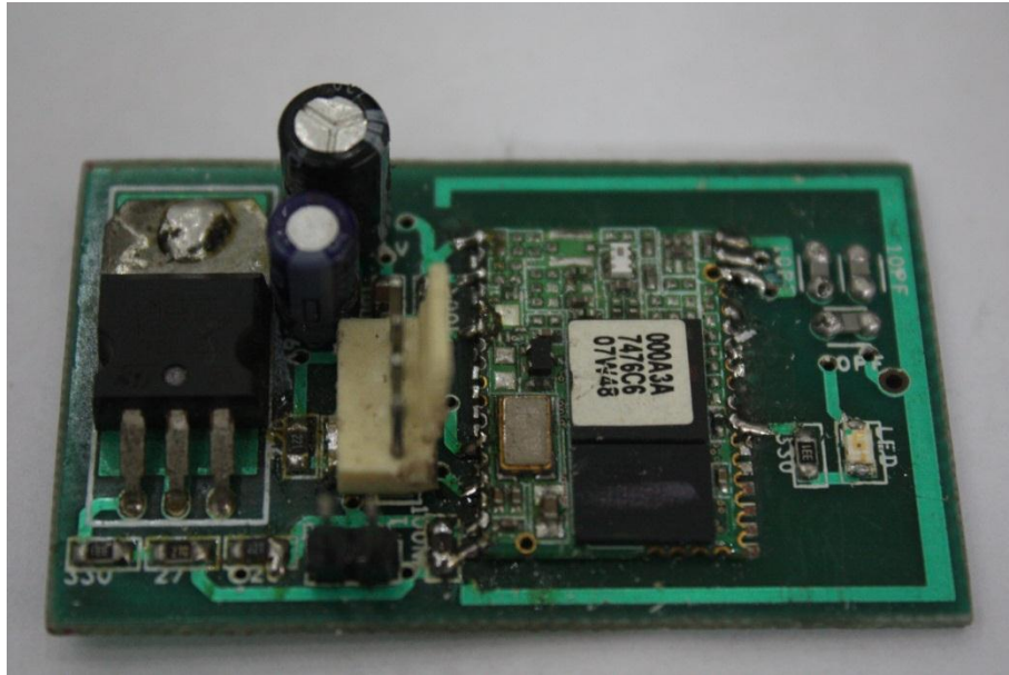
Modul Bluetooth DMB – 01
