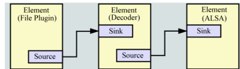
Fig. 1. GStreamer pipeline
