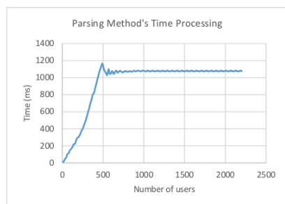
Figure 6. Parsing method's processing time graph
