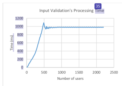
Figure 5. Input validation's processing time graph
