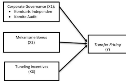
Figure 1 Research Model
