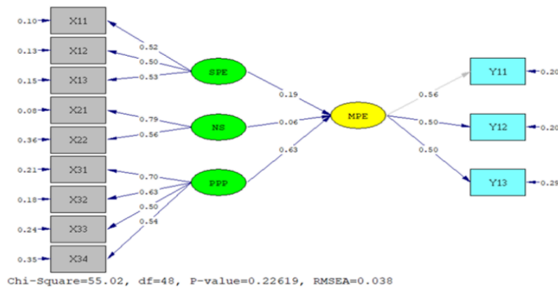
Gambar 2 : Diagram model factor
