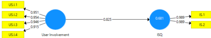
Fig. 2. Full Model Path Diagram
