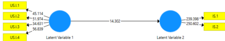
Fig. 1. Full Model T Statistics
