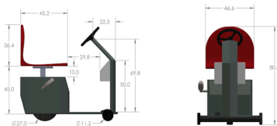
(a) Powered part side view (b) Powered part front view Figure 9. An elderly trolley with an elevated seat
