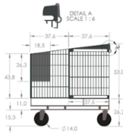
(b) Side view of basket part Figure 5. Basket part
