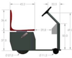
(b) Side view of powered part Figure 6. Powered part
