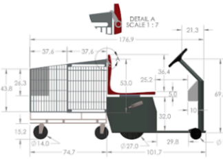
(b) Side view of both parts
