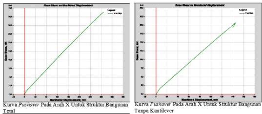
Gambar 9. Perbandingan kurva pushover arah X
