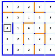
Figure 9. Simulation search path to cell (2,2)
