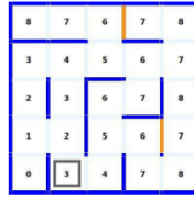
Figure 19. Simulation search path to cell (2,2)
