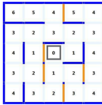
Figure 15. Simulation search path to cell (2,2)
