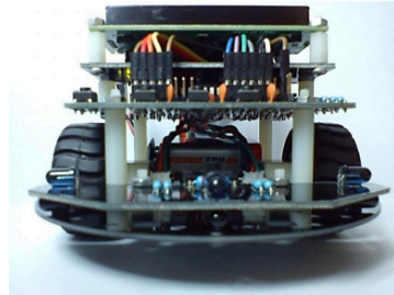
Figure 1. Mobile Robot from side view.
