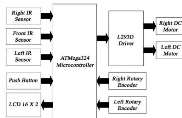
Figure 2. Block Diagram of Mobile Robot.
