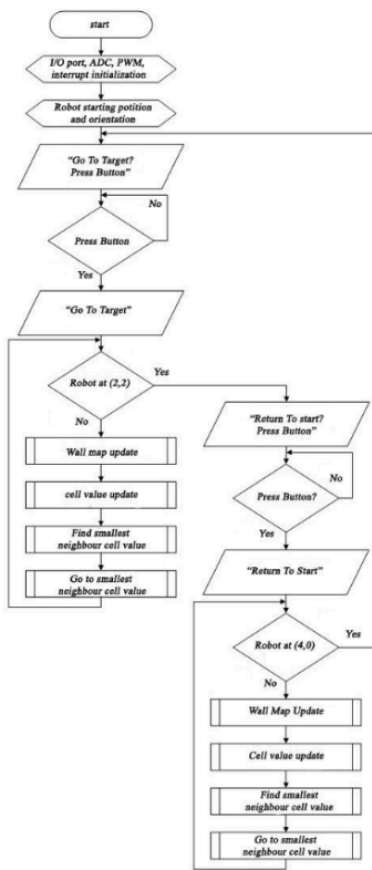
Figure 4. Flowchart of the main program.
