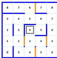
Figure 16. Simulation search path to cell (2,2)
