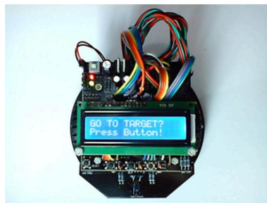
Figure 3. Mobile Robot from above view.
