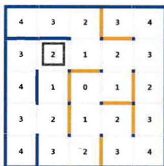
Figure 11. Simulation search path to cell (2,2)
