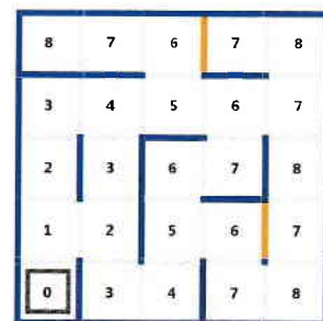
Figure 22. Simulation search path to cell (2,2)
