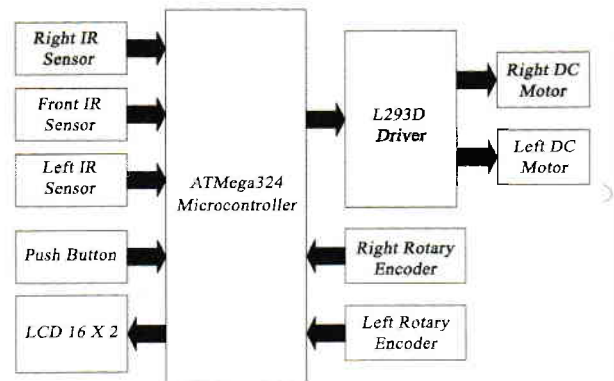
Figure 2. Block Diagram of Mobile Robot.
