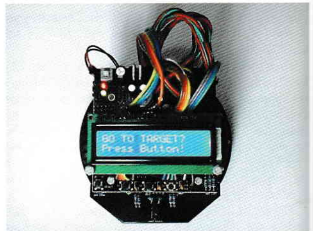
Figure 3. Mobile Robot from above view.
