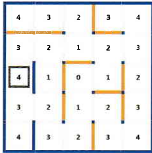
Figure 9. Simulation search path to cell (2,2)
