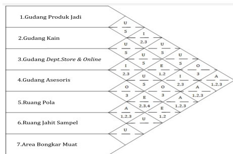
Gambar 3. Activity Relationship Chart (ARC)
