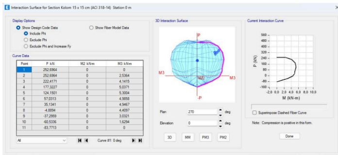
Fig. 11. Column interaction chart
