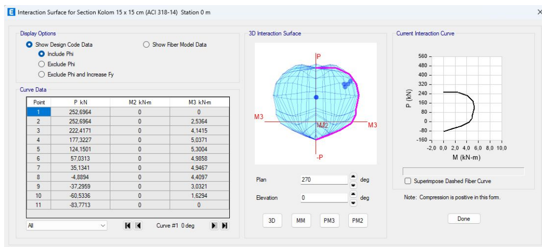
Fig. 11. Column interaction chart
