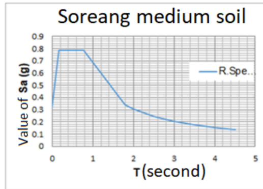
Fig. 12. Soil spectrum response diagram
