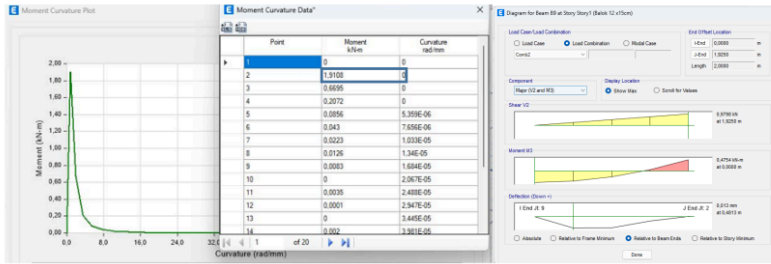
Fig. 10. Ultimate beam interaction and moment diagram
