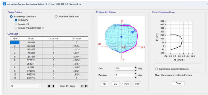
Fig. 11. Column interaction chart
