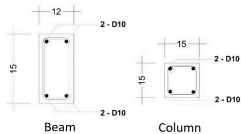
Fig. 6. Sections of columns and beams
