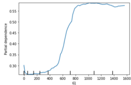
Gambar 14. PDP Total Spent on Website
