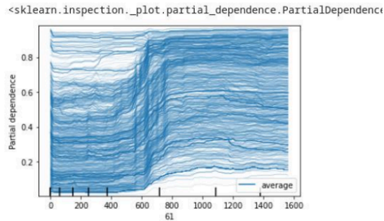
Gambar 17. ICE Total Time Spent on Website
