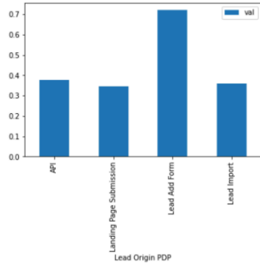
Gambar 15. PDP Lead Origin
