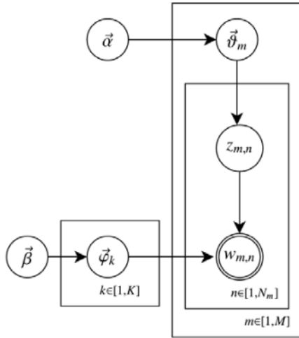
Fig. 2. Bayesian Network from Latent Dirichlet Allocation [10].
