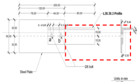
Fig. 4. Determine the clear distance (lc) hole to hole of bolts
