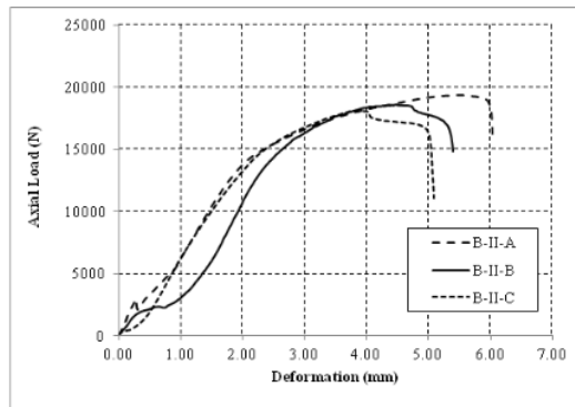
Fig. 9. P-D curves of Steel Axial Connection Specimen
