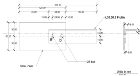
Fig. 3. Configuration of axial tensile steel connection
