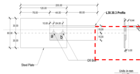
Fig. 5. Determining the block shear
