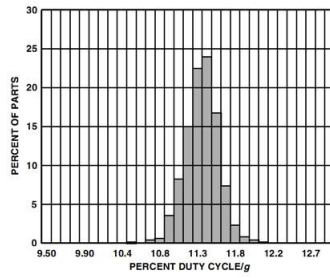
TPC 8. X-Axis Sensitivity at X_{OUT} , V_{DD} = 3\text{ V}
