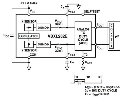
Figure 3. Block Diagram
