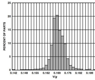
TPC 7. Y-Axis Sensitivity Distribution at Y_{FILT} , V_{DD} = 3\text{ V}
