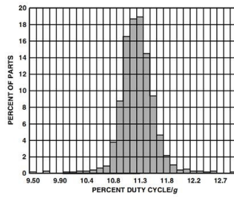
TPC 9. Y-axis Sensitivity at Y_{OUT} , V_{DD} = 3\text{ V}
