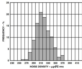
TPC 13. Noise Density Distribution, V_{DD} = 3\text{ V}
