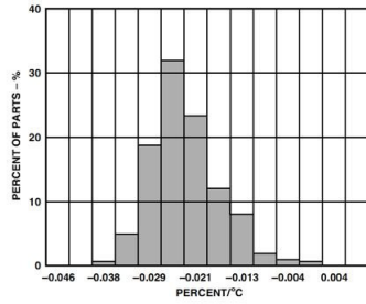
TPC 20. X-Axis Sensitivity Drift at X_{\text{FILT}} Due to Temperature Distribution, -40^{\circ}\text{C} to +85^{\circ}\text{C}
