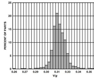
TPC 10. Y-Axis Sensitivity Distribution at Y_{FILT} , V_{DD} = 5\text{ V}
