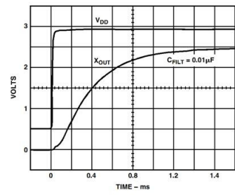
TPC 18. Typical Turn-On Time
