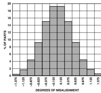
TPC 15. Rotational Die Alignment
