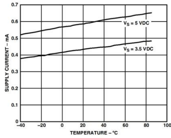
TPC 14. Typical Supply Current vs. Temperature
