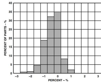
TPC 17. Cross-Axis Sensitivity Distribution
