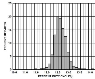
TPC 12. Y-axis Sensitivity at Y_{OUT} , V_{DD} = 5\text{ V}
