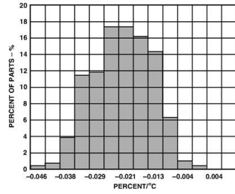
TPC 23. Y-Axis Sensitivity Drift at Y_{\text{FILT}} Due to Temperature Distribution, -40^{\circ}\text{C} to +85^{\circ}\text{C}
