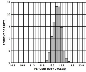
TPC 11. X-Axis Sensitivity at X_{OUT} , V_{DD} = 5\text{ V}
