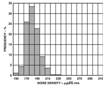
TPC 16. Noise Density Distribution, V_{DD} = 5\text{ V}
