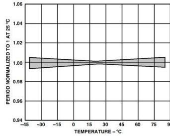
TPC 25. Normalized DCM Period (T2) vs. Temperature
