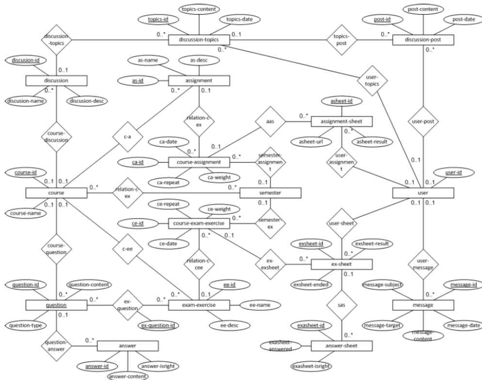
Gambar 6 Entity Relationship Model Struktur Data Aplikasi E-learning
