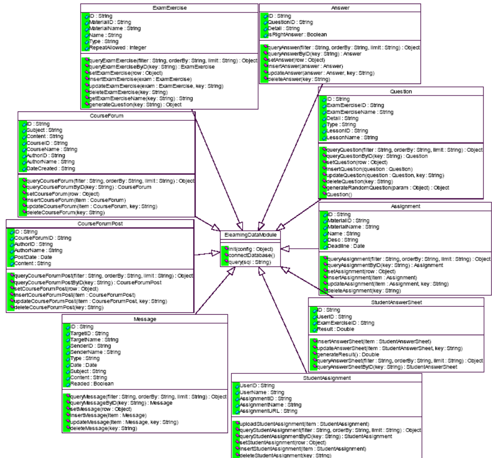
Gambar 5 Class Diagram Objek ElearningDataModule
