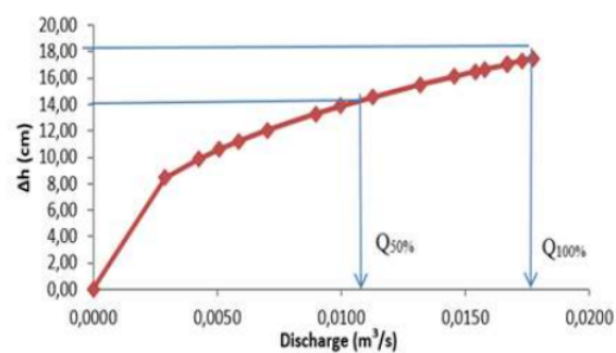
Figure 6. Rating curve.
