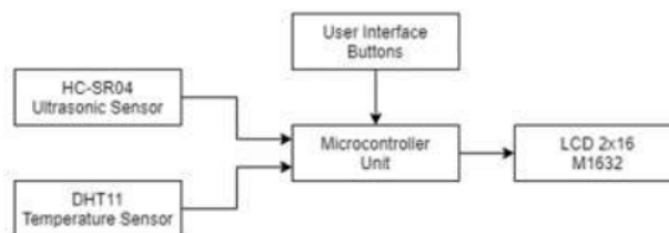
Figure 5. Measurement device block diagram.
