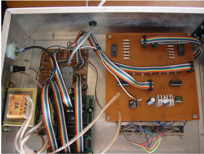
Rangkaian MCS-51
