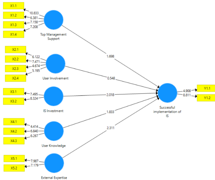
Figure 2. Full Model T-Statistics
