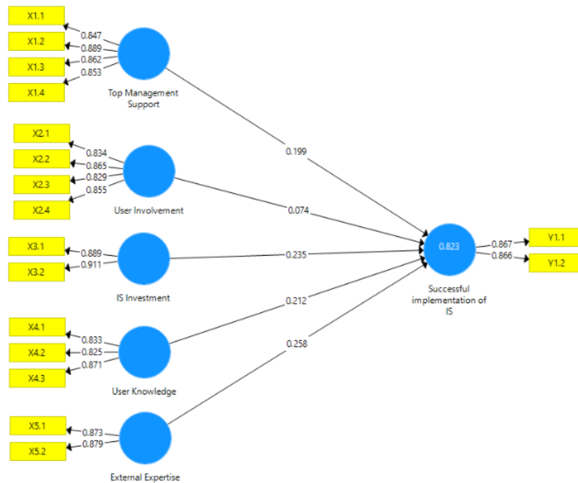
Figure 1. Full Model Path Diagram
