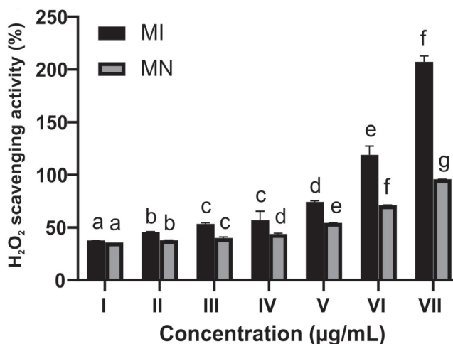
Figure 5: Percentage of H 2 O 2 scavenging activity in mangosteen and mangosteen nanoemulsion
