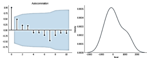
Gambar 15. Plot autokorelasi dan histogram model seasonal naive visitor
