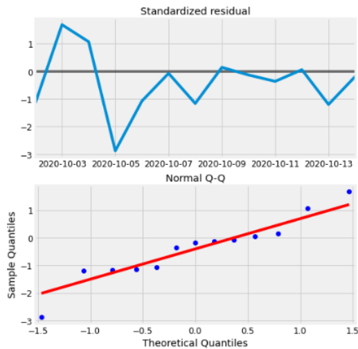
Gambar 10. Plot Residual dan Plot QQ model data visitor
