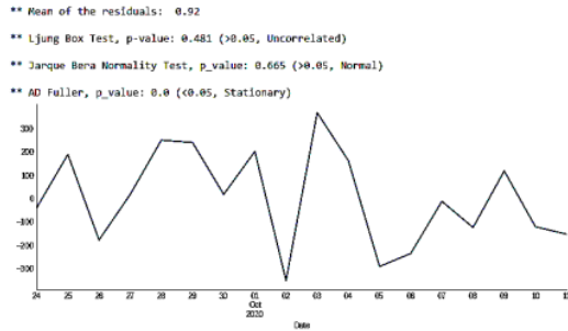
Gambar 18. Distribusi residual model Holt Winter visitor
