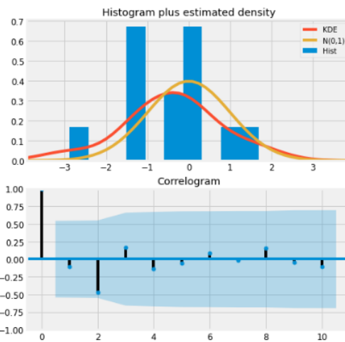
Gambar 9. Histogram dan Correlogram model visitor
