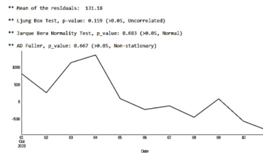
Gambar 14. Distribusi residual model
