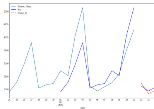
Gambar 13. Visualisasi seasonal naive Forecast
