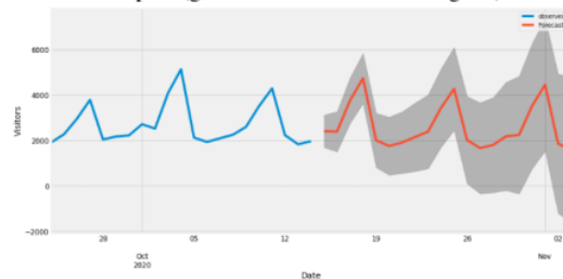
Gambar 12. Visualisasi prediksi seasonality data
