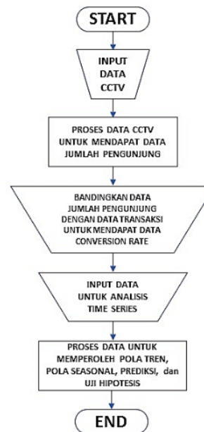
Gambar 2. Flowchart penelitian
