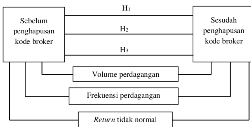
Gambar 1 Riset Model
