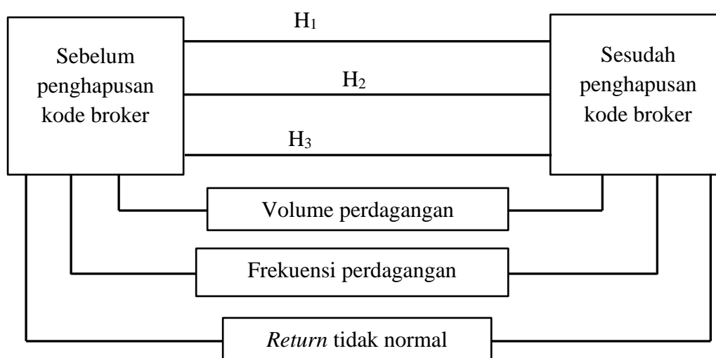
Gambar 1 Model Penelitian
