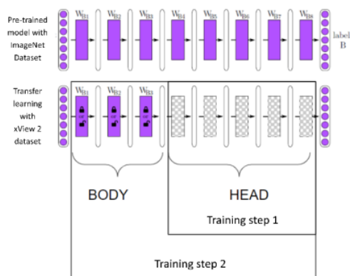
Figure 4. Transfer learning approach illustration
