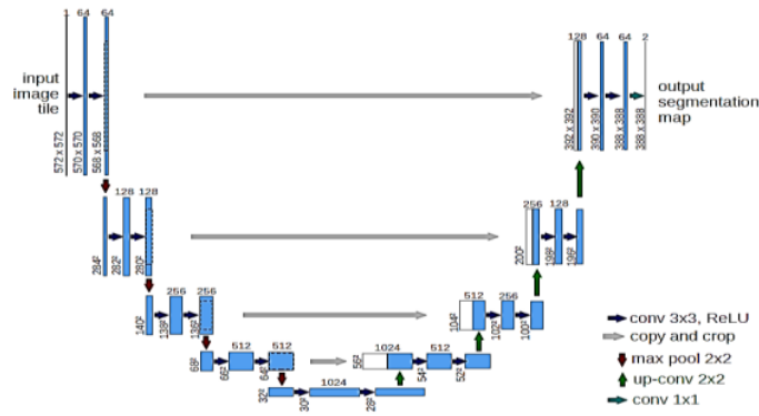
Figure 1. U-Net architecture [10]
