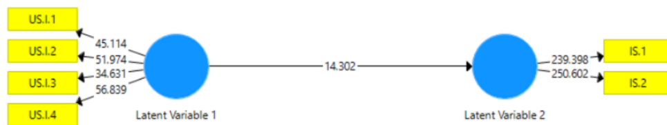
Fig. 1. Full Model T Statistics
