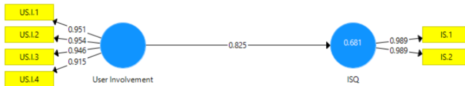
Fig. 2. Full Model Path Diagram
