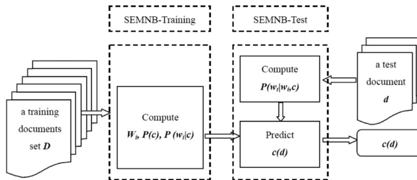
Figure 3: SEMNB algorithm framework [4].
