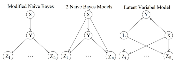
Figure 1: Three Naïve Bayesian Approaches.
