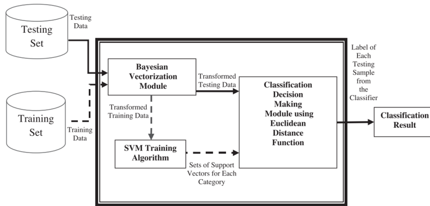
Figure 2: SVM-NN [13].
