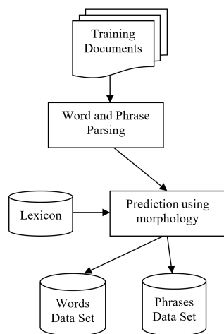
Figure 4: Training Process.
