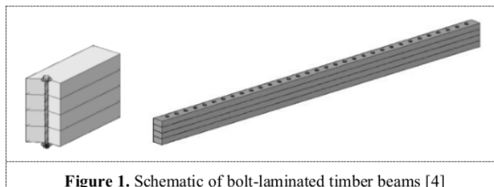
Figure 1. Schematic of bolt-laminated timber beams [4]
