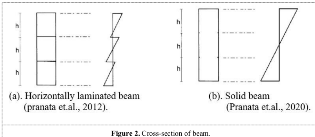
Figure 2. Cross-section of beam.
