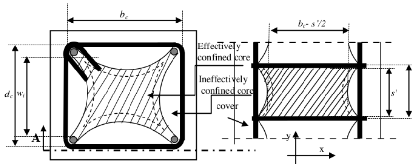
Figure 2 Effectively confined core for rectangular hoop reinforcement.
