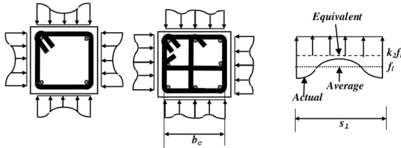
Figure 3 Lateral pressure in a square column [6].
