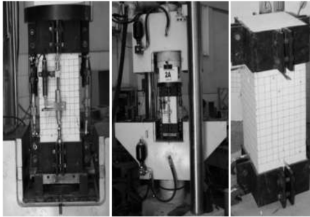
Figure 7 Specimen, test setup and compression testing machine.
