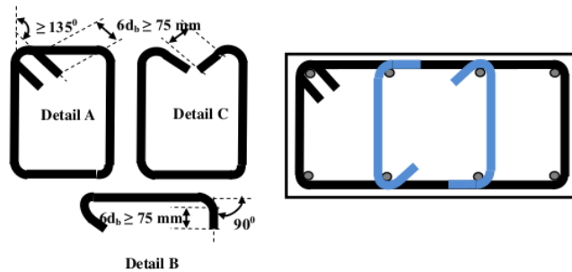
Figure 1 Seismic hook detailing.
