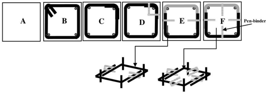
Figure 5 Confining reinforcement configurations.
