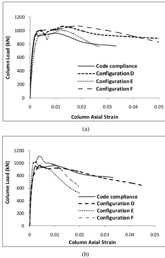
Figure 8 Axial load-strain relationship of average between two specimens with various confinement configurations, (a) steel pen-binder, (b) plastic pen-binder.
