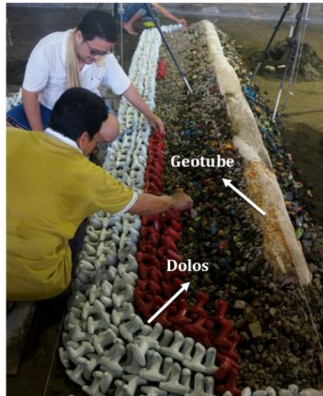
Figure 2. Process of establishing the rubble-mound breakwater model
