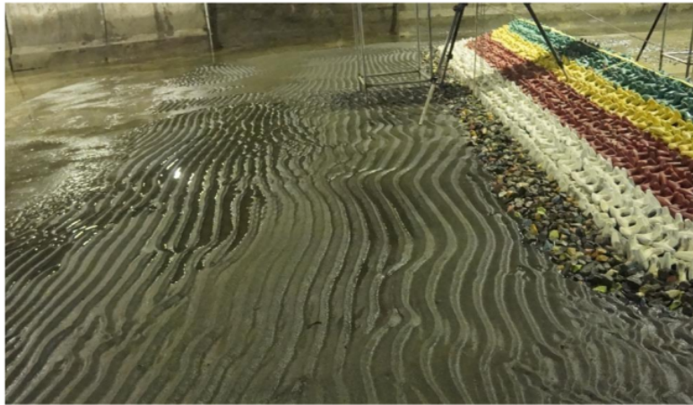
Figure 11. Sediment condition after loaded with daily waves simulation
