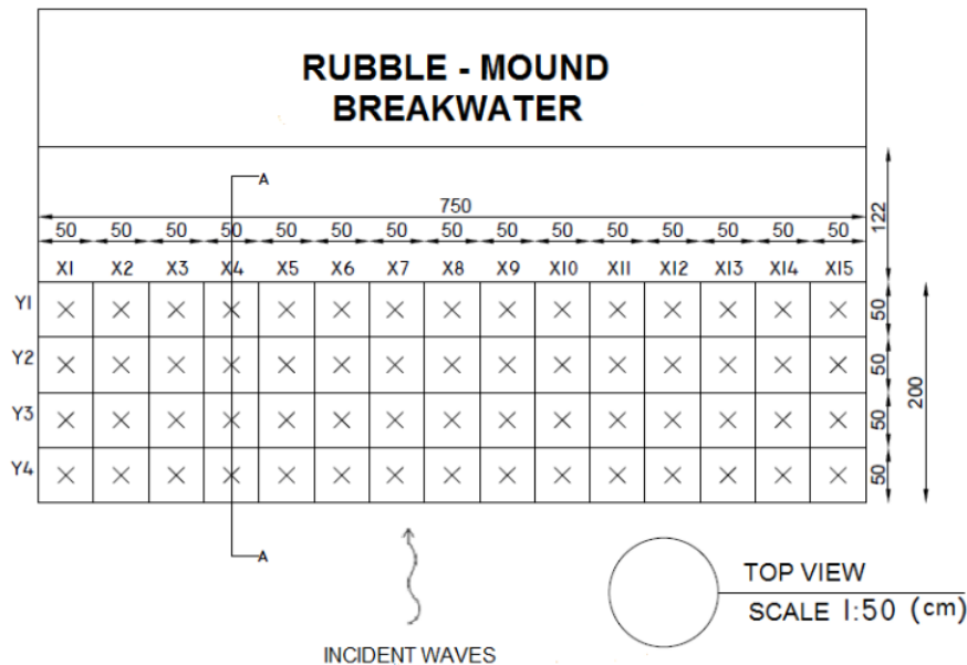
Figure 5. Sedimentation research points
