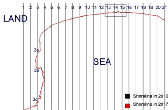
Figure 11: Coastlines in the year 2016 and 2017.
