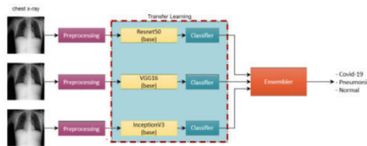
Fig. 1. Deep Learning Ensemble Model Block Diagram
