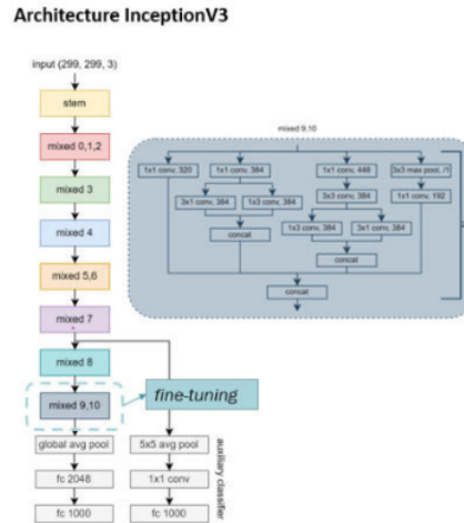
Fig. 5. InceptionV3 Architecture Diagram (fine-tuning)
