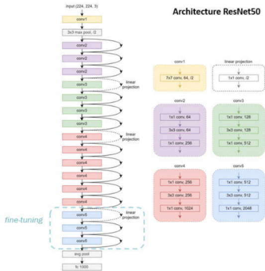
Fig. 3. ResNet50 Architecture Diagram (fine-tuning)
