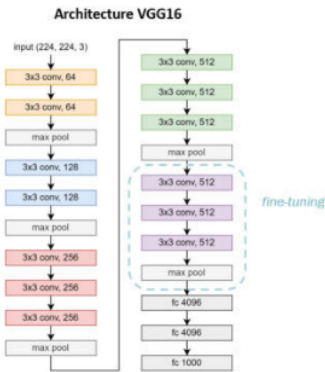
Fig. 4. VGG16 Architecture Diagram (fine-tuning)
