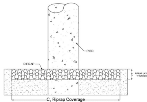
Figure 2: Detail sketch of the riprap layer.
