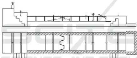
Figure 1: Experimental set up (top view and side view).
