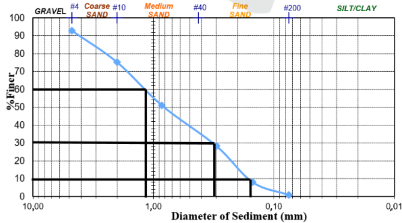
Figure 2: Sieve analysis results.
