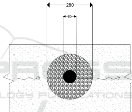
Figure 4: Illustration of riprap with circular shape (top view, unit: mm).
