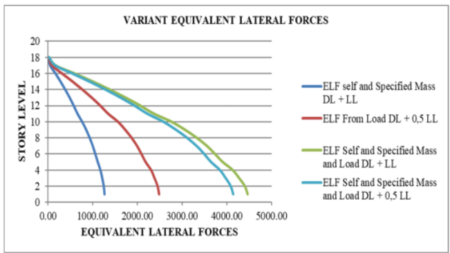
Figure 3: Variation of equivalent lateral forces.
