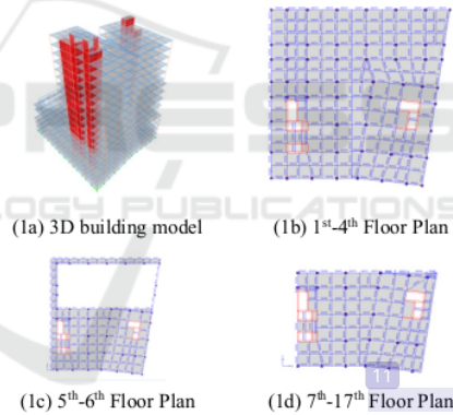
Figure 1: Building model and floor plane data.
