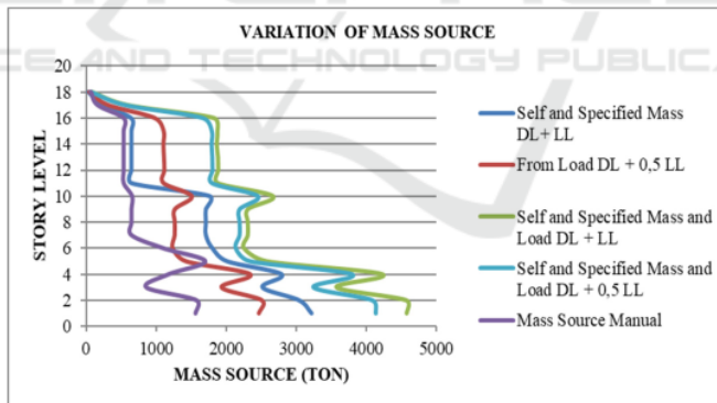
Figure 2: Variation of mass source.
