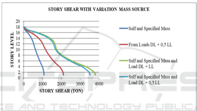
Figure 4: Story shear with variation mass source.
