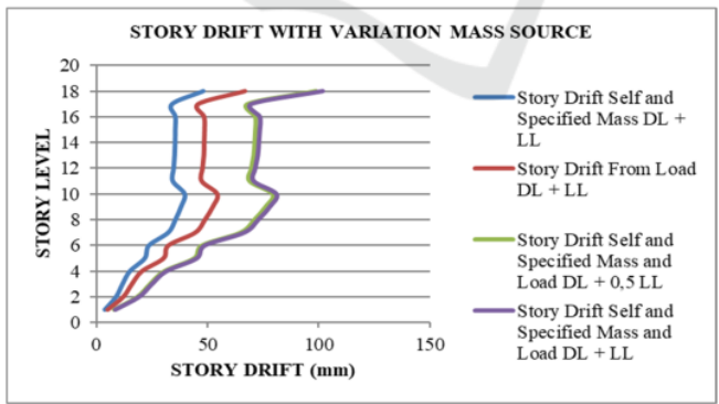
Figure 5: Story drift with variation mass source.
