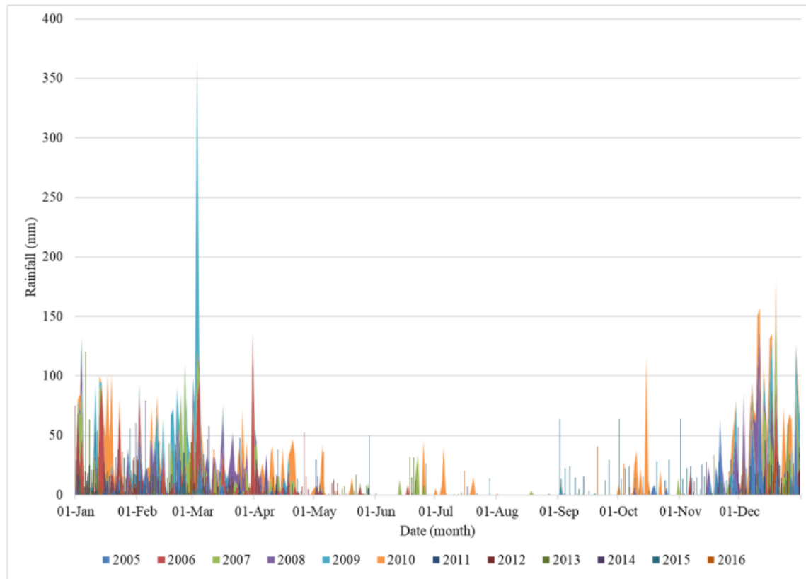
Fig. 2. Daily rainfall data (2005–2016) at Tardamu rain gauge, Savu Rai Jua.
