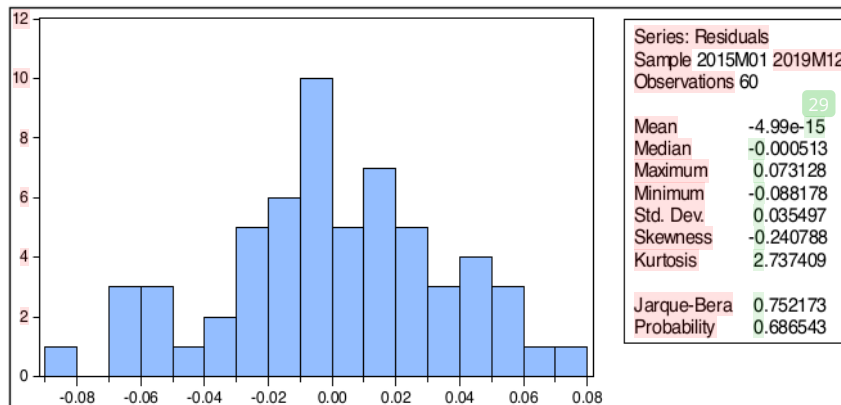
Figure 1. Normality Test
