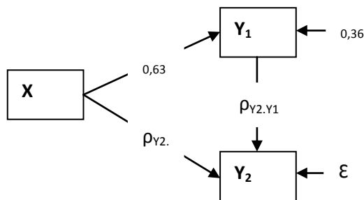
Gambar 4 Diagram Path
