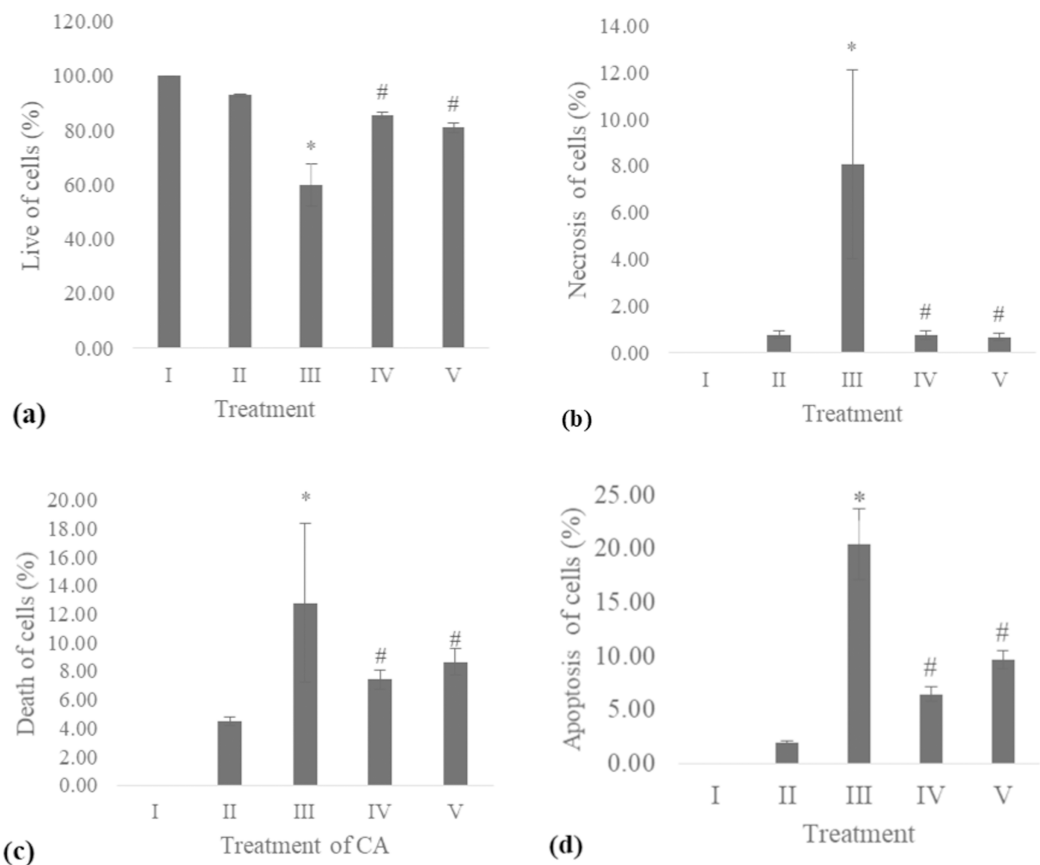
Figure 5 Effect CA towards apoptosis cells on UV-induced fibroblast cells. (A) live of cells, (B) necrosis of cells, (C) death of cells (late apoptosis of cells), (D) apoptosis of cells (early apoptosis of cells) (I) BJ cells (negative control), (II) BJ cells + DMSO 1% (vehicle control), (III) BJ cells + UV (positive control), (IV) UV-induced BJ cells + CA cells + CA 6.25 \mu\text{g/ml} , (V) UV-induced BJ cells + CA 25 \mu\text{g/ml} . *Data is presented as mean \pm standard deviation. A single asterisk symbol (*) marks statistical difference compared to negative control group at 0.05 significance level, a single hashtag (#) marks statistical difference compared positive control at 0.05 significance level based on Tukey HSD post hoc test.
