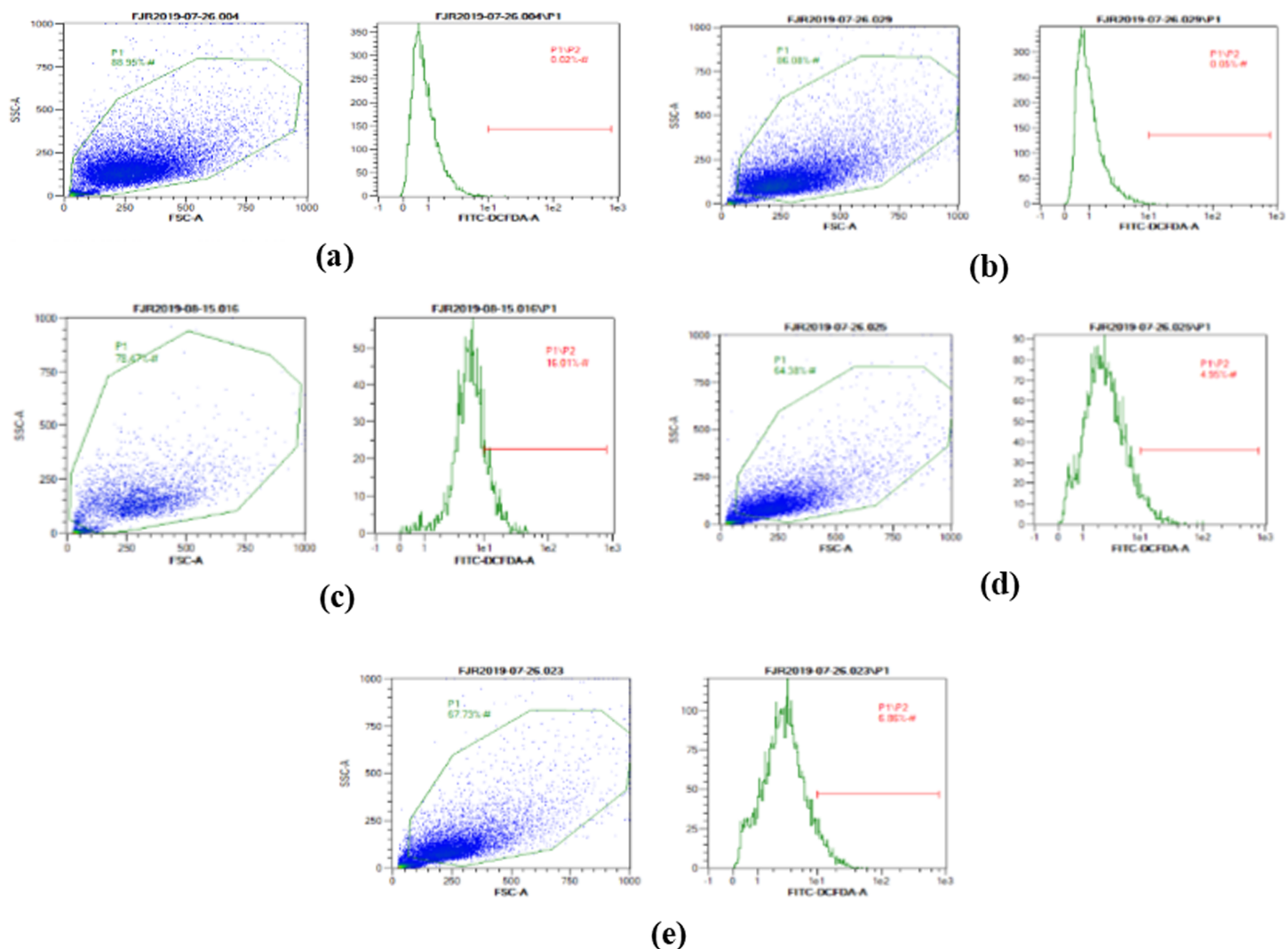
Figure 2 The representative of dot blots of various concentration CA on UV-induced fibroblast cell toward ROS level by flow cytometry. (A) BJ cells (negative control); 0.02%, (B) BJ cells + DMSO 1% (vehicle control): 0.05%, (C) BJ cells + UV (positive control): 16.01%, (D): UV-induced BJ cells + CA 6.25 µg/ml: 4.95%, (E): UV-induced BJ cells + CA 25 µg/ml: 6.86%. Full-size DOI: 10.7717/peerj.11419/fig-2
