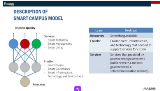
Fig 9. Description Smart Campus Model
