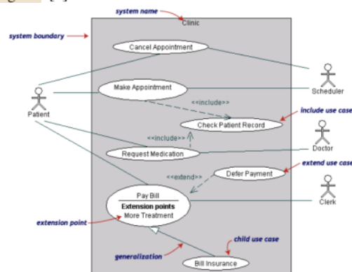
Figure 1 Example of Use Case Diagram
