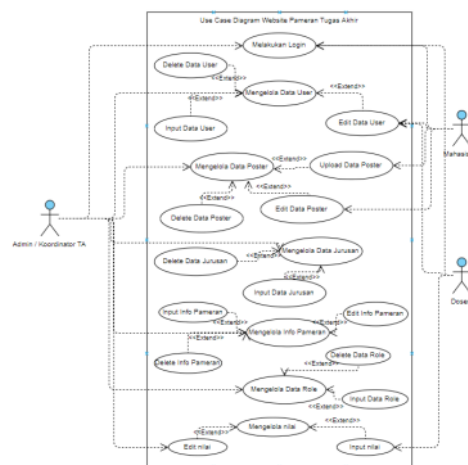
Figure 2 Use Case Diagram of Final Project Exhibition Website
