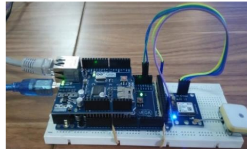
Figure 4. GPS NTP server based on arduino mega 2560
