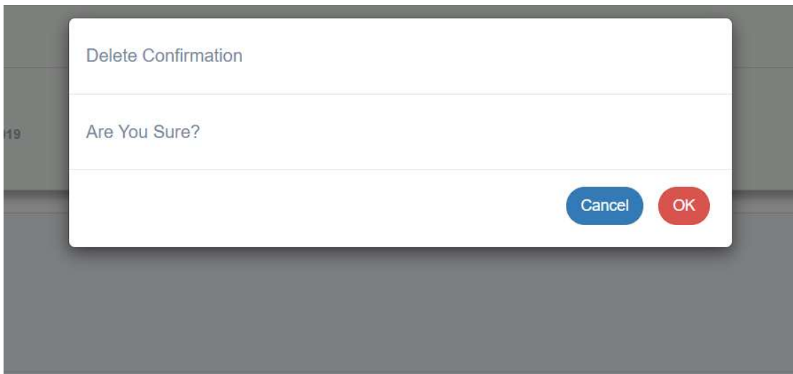
Gambar 3.6 Delete Reply
