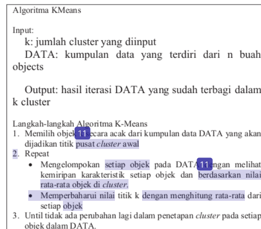
Gambar 1 Algoritma KMeans [2]
