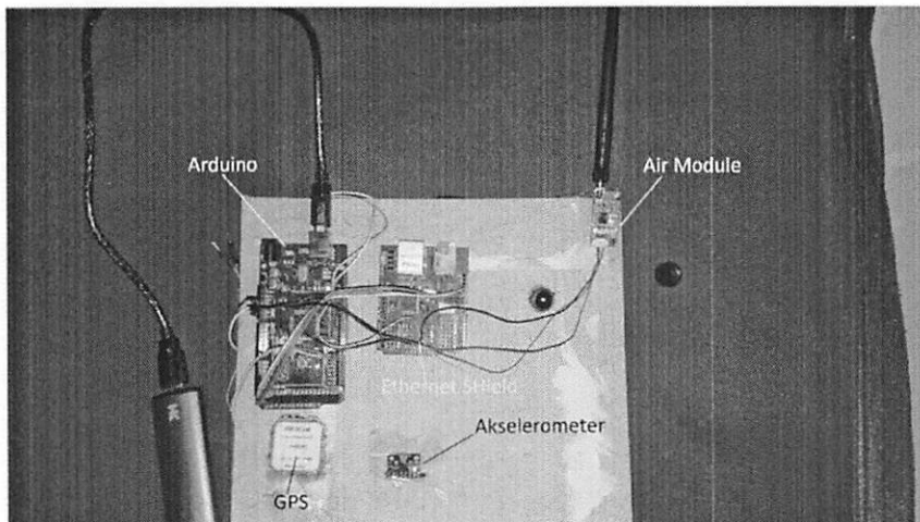
Gambar 9 Realisasi Hardware Pengirim
