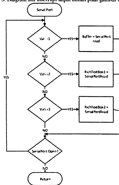
Gambar 8 Diagram Alir Interrupt
