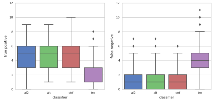
Fig. 10. Comparison of true positive and false negative detections among four pre-trained classifiers toward our gold standard dataset .
