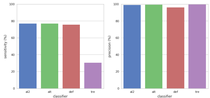
Fig. 11. Measure of sensitivity and precision across the four pre-trained classifiers toward our gold standard dataset .
